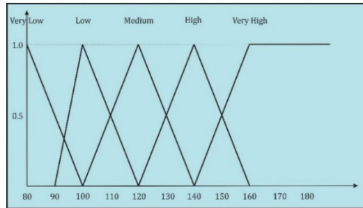
Fig. 6. Membership Functions of the Output Variable “Average Energy Consumption”
