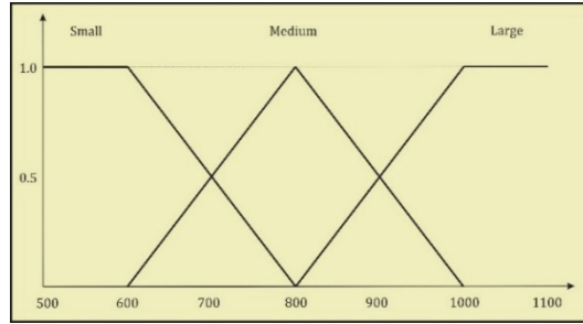
Fig. 5. Membership Functions of “Non-Productive Kilometres” Fuzzy Variable
