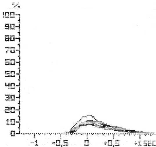
Fig. 6. The Emissions from Motor Mercedes Benz Actros, Collected on the Field with Testing
